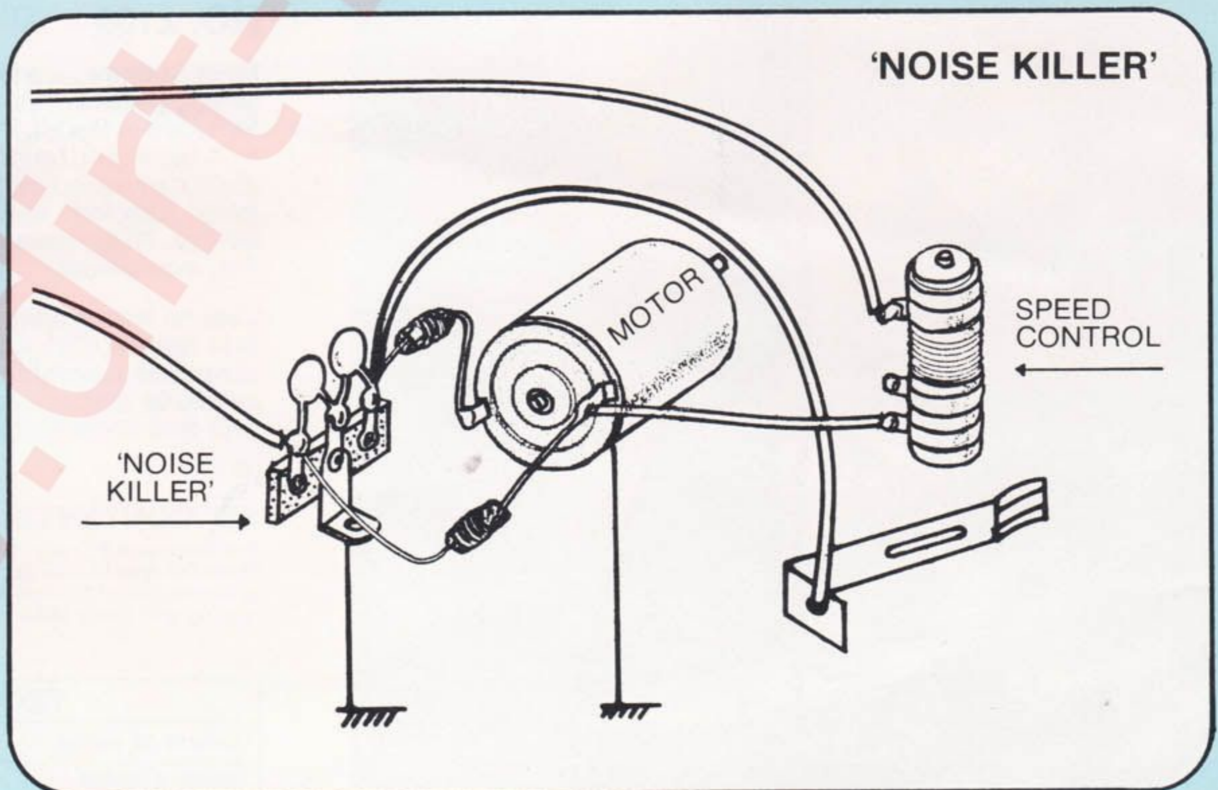
Typical Hook-up Of Accessories To Motor
